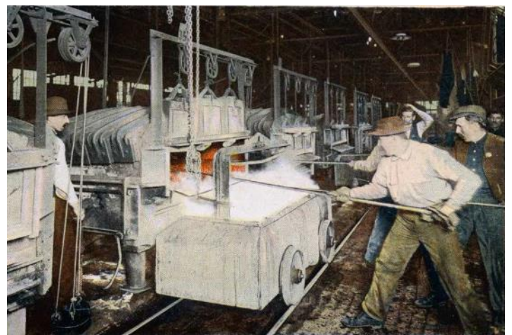
"Quenching steel forgings in the furnace room. Ford heat treatment gives wonderful strength to axles, steering rods, gears etc."
